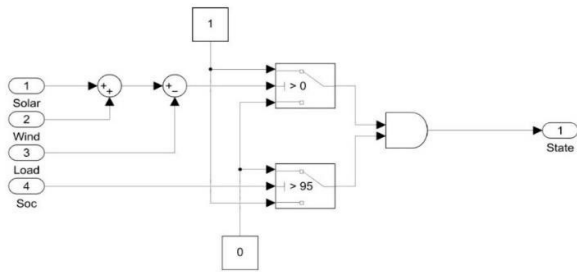
Fig. 14. Figure of Battery Logic
