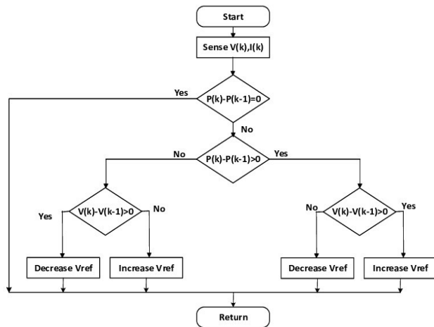
Fig.2. P&O method flow chart
