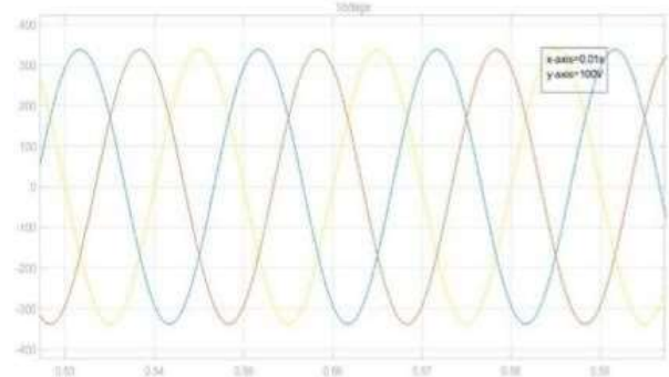
Fig.25. Voltage graph of the PCC
