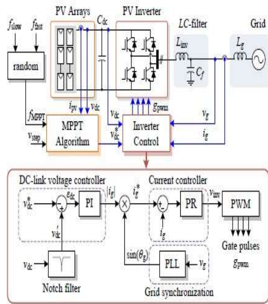
Fig. 1. System diagram and control structure of single-stage single-phase PV inverter (PI - Proportional Integral, PR - Proportional Resonant, PWM - Pulse Width Modulation, PLL - Phase-Locked Loop).
