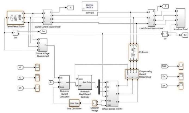
Fig.5: Simulink model of PSQPI theory
