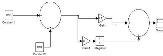
Fig.4: Simulation block of PSO based PI controller
