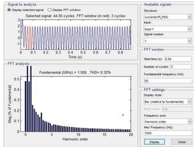
f) %THD in Current with PSO-PI controller
