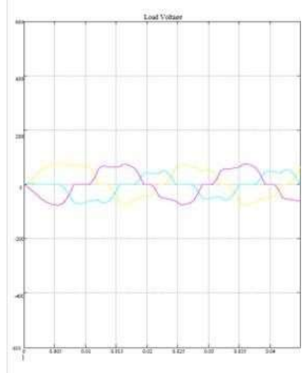
d) Three Phase Load Voltage Using SAPF
