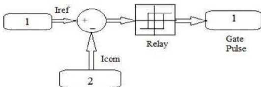
Fig.2: Hysteresis band current controller
