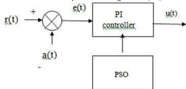
Fig.3: Block diagram of PSO based PI controller
